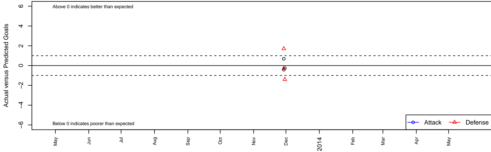
San Diego Surf SC Premier I G01 Dots are actual minus expected GF (blue circles) and GA (red triangles). Blue line is smoothed change in attack strength. Red is smoothed change in defense strength.
